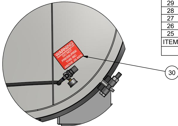
DETAIL E
